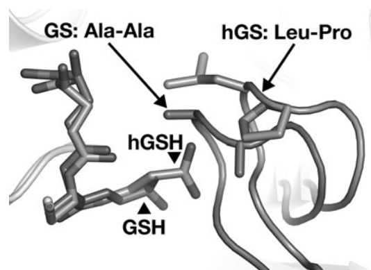
Fig. 4 Comparison of glutathione ( GSH ) and homogluthatione ( hGSH ) binding in the active sites of glutathione synthetase ( GS ) and homogluthatione synthetase ( hGS ). The active site loop differences determining substrate specificity of GS ( Ala-Ala ) and hGS ( Leu-Pro ) are indicated by the arrows. Modified from Galant et al. 2009
